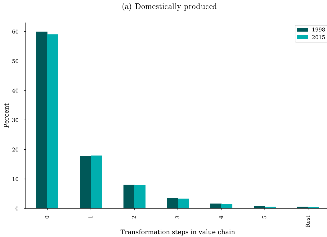
Figure 6: Length of value chain for requirements of a dollar of PCE (1998 and 2015)
