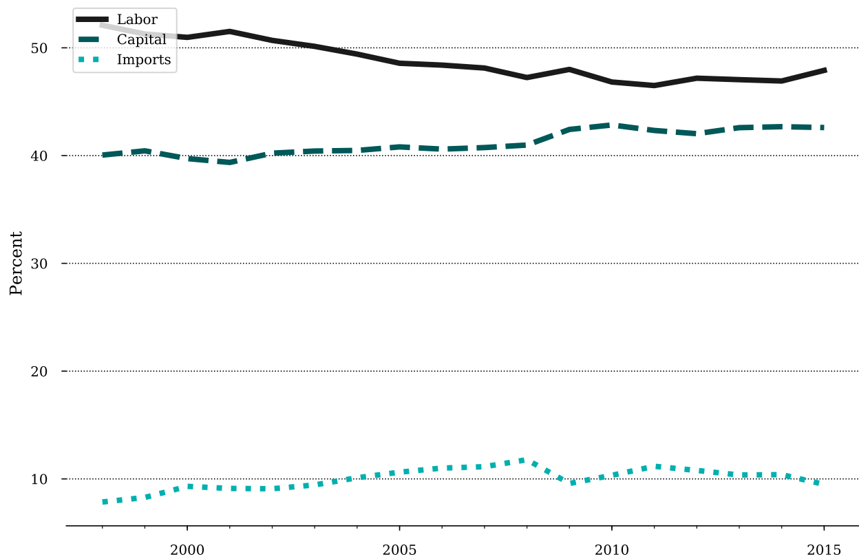
Figure 7: Factor requirements of a dollar of PCE.
