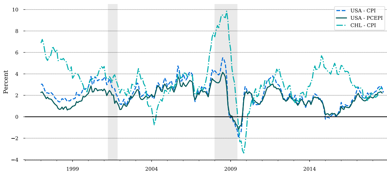
Figure 1: Inflation rates in U.S. and Chile: 1996-2018.
