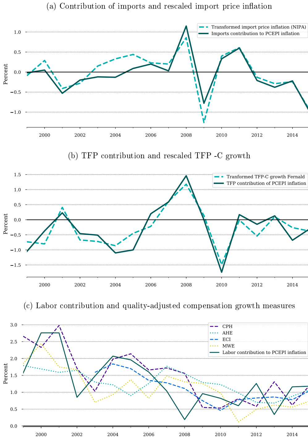
Figure 11: Real-time rule-of-thumb approximation of “supply-side origins” of inflation.
