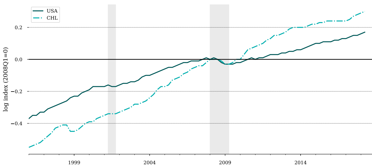
Figure 2: Log real GDP in U.S. and Chile: 1996-2018.
