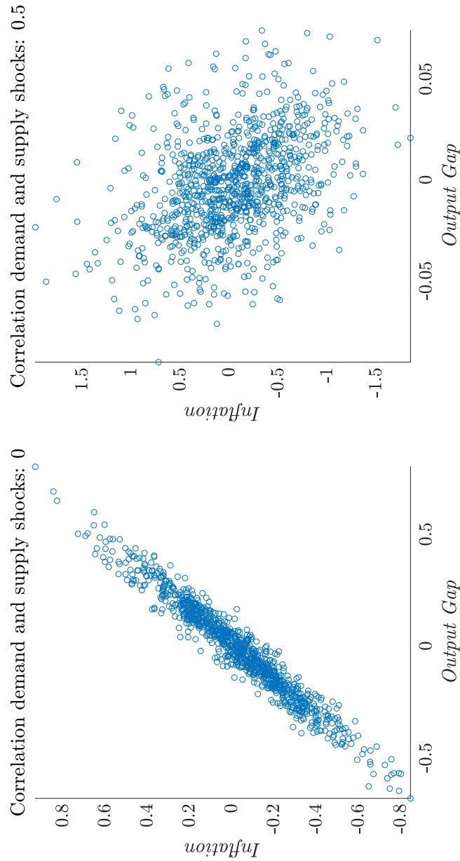
Figure 4: Phillips Curve in NK-model with uncorrelated and correlated shock
