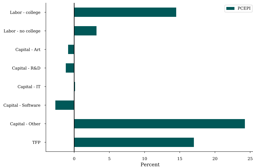
Figure 9: Variance decomposition of annual PCEPI inflation for production factors.
