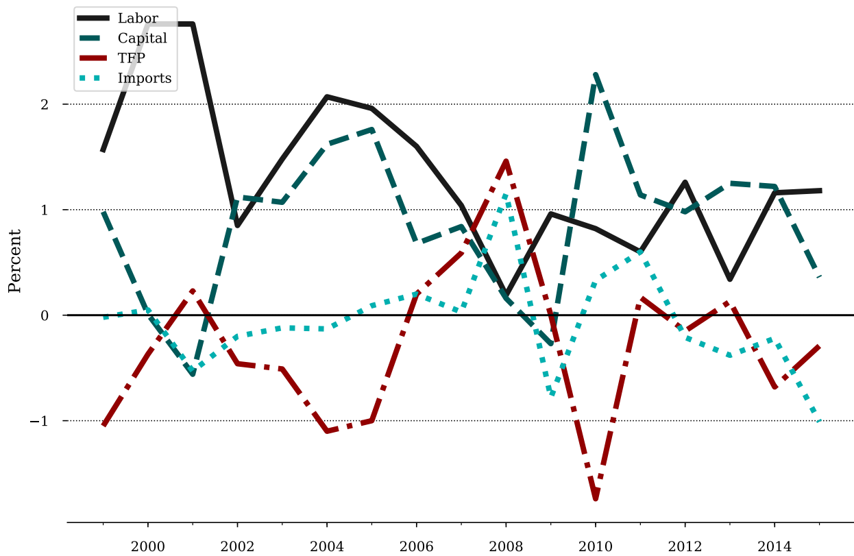
Figure 10: Factor contributions to annual PCEPI inflation.
